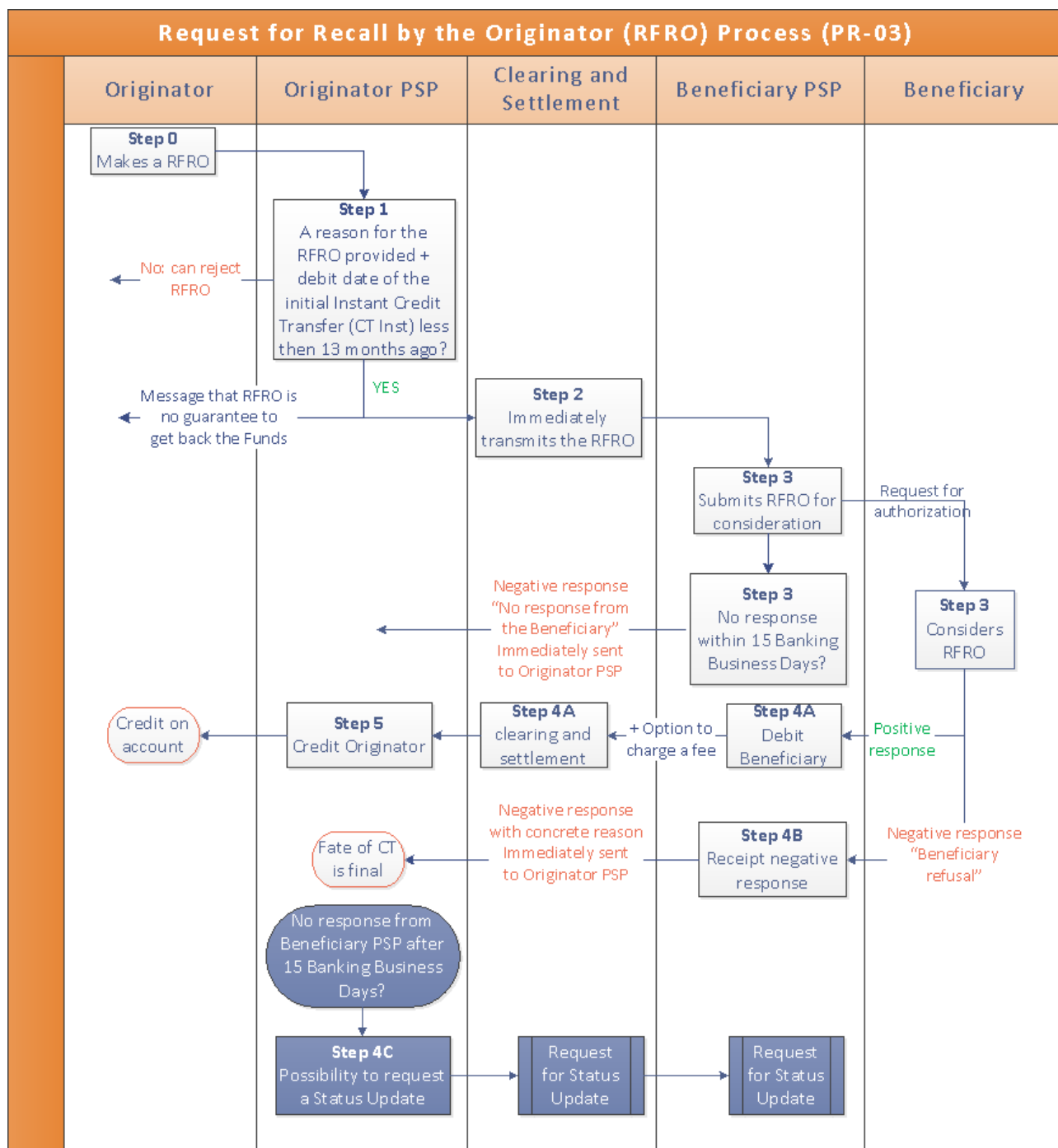
Figure 8: SCT Inst Request for Recall by the Originator Process (PR-03)
